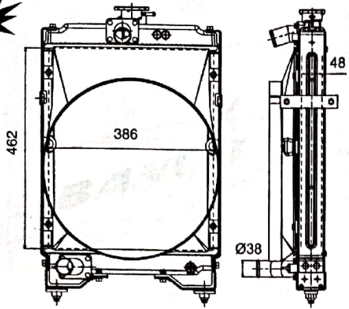
TAFE CHALLENGER Core - B-8124302029ALU
