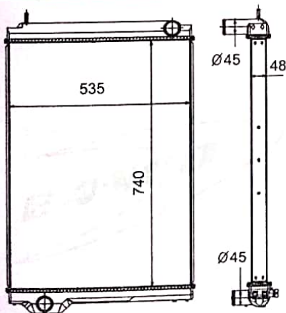
A/L 4018/3518/3516/2516/412 AC/TC BS-II (BOLT TYPE) CORE - B-8360842029ALU
