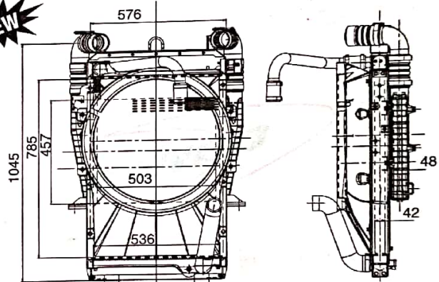
TATA TML LPS 4018 BS-IV AC RADIATOR ASSEMBLY (SIGNA) CAC - 8220842010CAC
