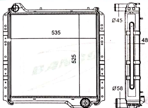
TATA 697 CMVR BRASS O/F PIPE WITH 8 HOLE SIDE FRAME CORE - B-8220902029ALU
