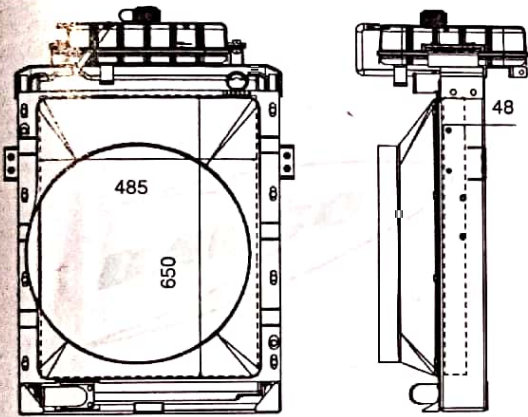
A/L GOODS ETI ENG. BS-II RADIATOR - B-8360732020ALU, CORE - B-8360732029ALU, B-8360732020RWC, Rad.+SF+MF+Shroud+DAT+CAC CAC - 8360732010CAC
