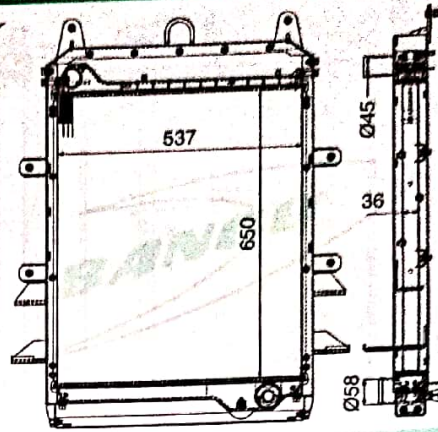
TATA 4018 VAVE RADIATOR ASSY. Radiator - 8220822080ALU Radiator - 8220822070ALU, W/ SF CAC - 8220822010CAC
