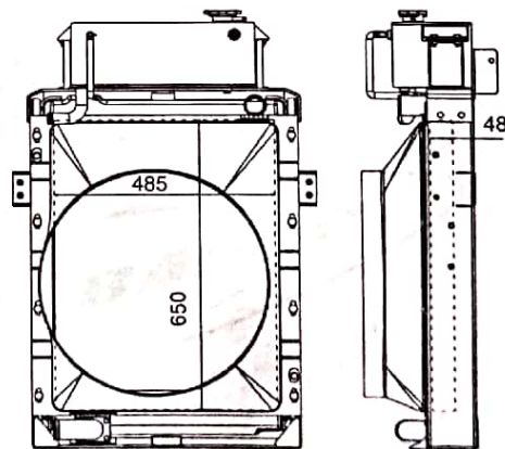
A/L PASSENGER 6 ETI ENG. WITH CAC (BS-II) / H6ET RADIATOR - B-8360712020ALU, CORE - B-8360712029ALU, B-8360712020RWC, Rad.+SF+MF+Shroud+DAT+CAC CAC - 8360712010CAC
