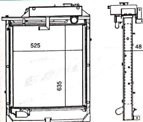
A/L PASSENGER BS-I WITH DAT CORE - B-8360772029ALU
