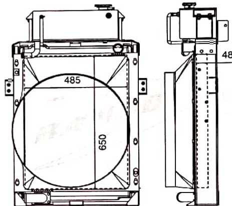
A/L PASSENGER DTI ENG. RADIATOR - B-8360702020ALU, CORE - B-8360702029ALU, B-8360702020RWC, Rad.+SF+MF+Shroud+DAT+CAC CAC - 8360702010CAC
