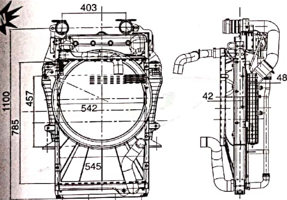
TATA TML LPT 3118/LPT3718 AC BS-IV RADIATOR ASSEMBLY (AJINKYA) CAC - 8220832010CAC
