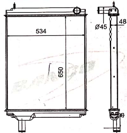
A/L 412 ACTC WITH NEW BOTTOM TANK (B II-268) CORE - B-8360822029ALU
